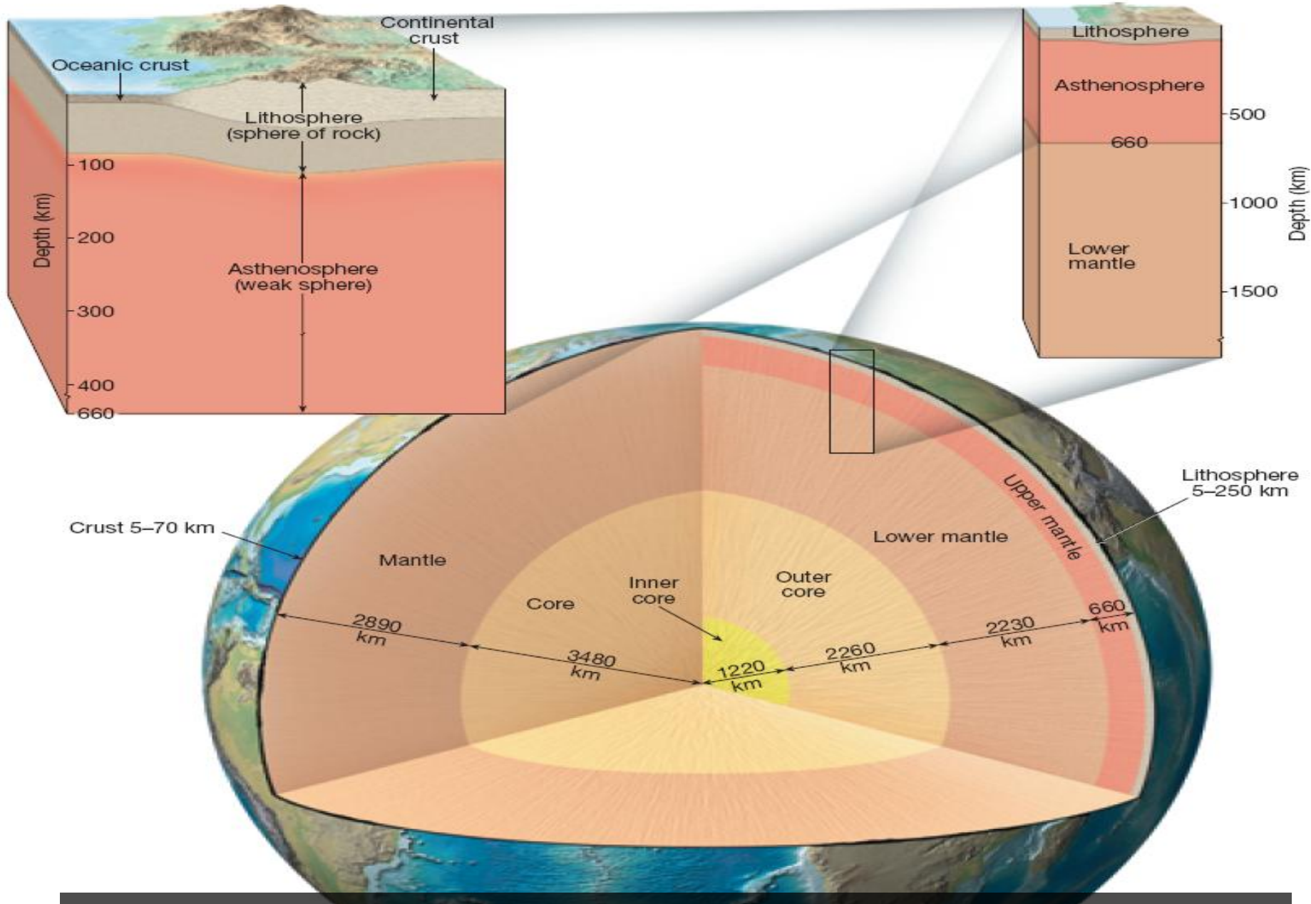
Earth's Layered Structure.
